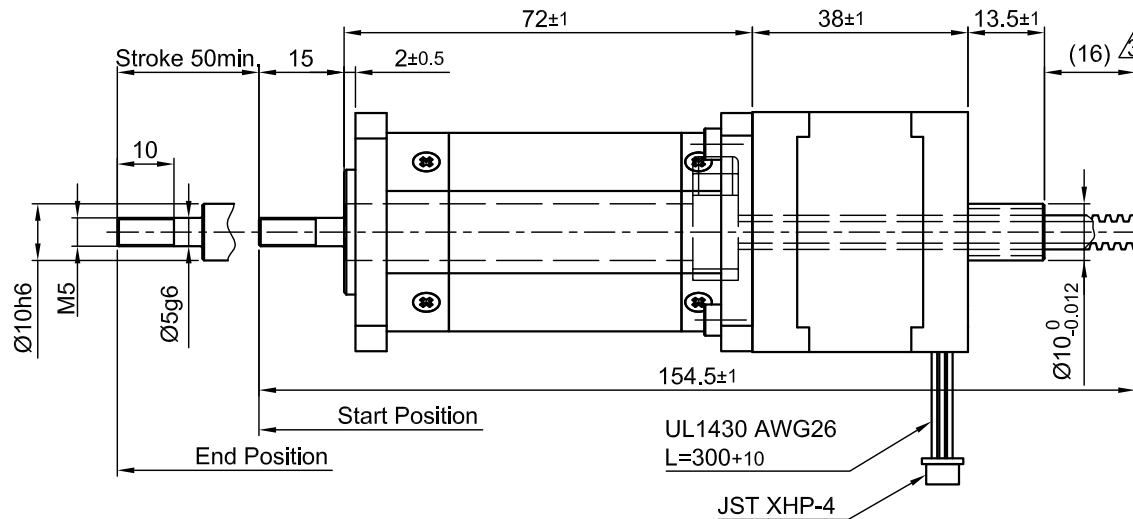
Side view
