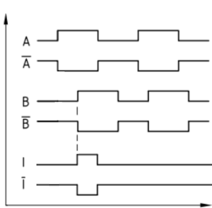
Fig. 5: Clockwise (viewing the motor drive shaft), the channel A signal precedes channel B by 90° (electrically). The index signal is 90° wide and synchronous to the channel B edge.
