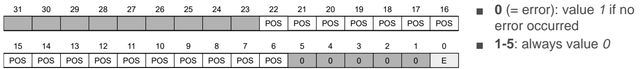
Fig. 8: NME2 transfers 23 bits: E for error, 17 POS for position, 5 zero bits
