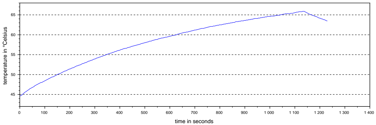
PD2-CB: Controller temperature at 45° Celsius ambient temperature and 3.3A motor current
