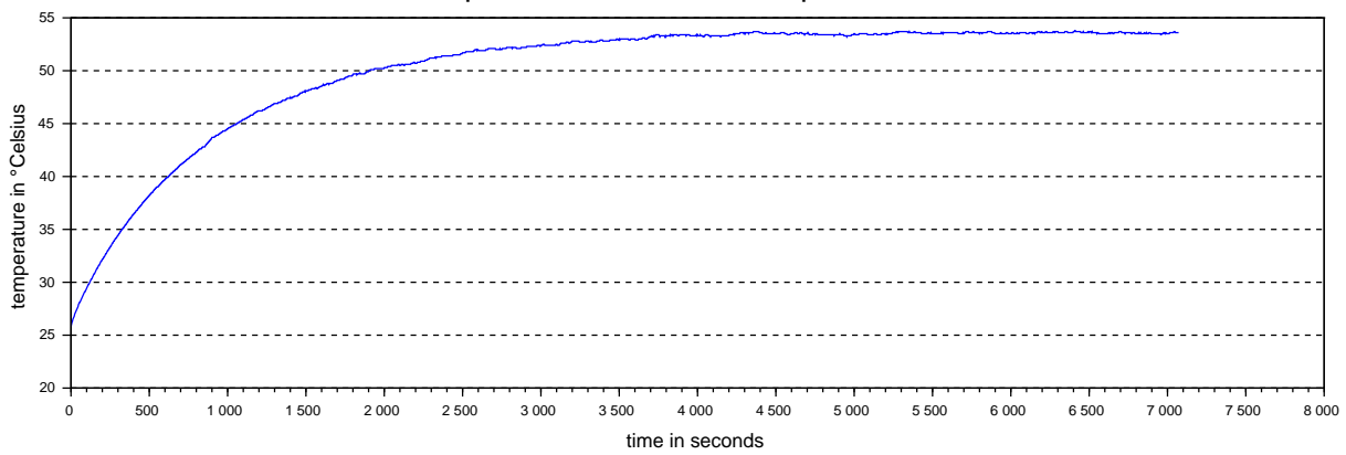
PD2-CB: Controller temperature at 25° Celsius ambient temperature and 3.3A motor current
