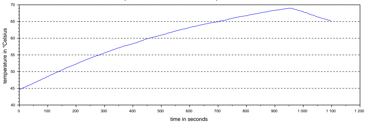
PD2-C: Controller temperature at 45° Celsius ambient temperature and 1.8A motor current
