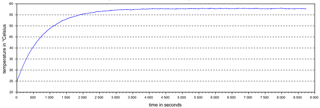
PD2-C: Controller temperature at 25° Celsius ambient temperature and 1.8A motor current
