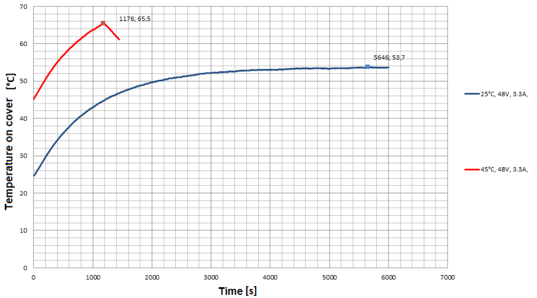
PD2-CB Temperature
