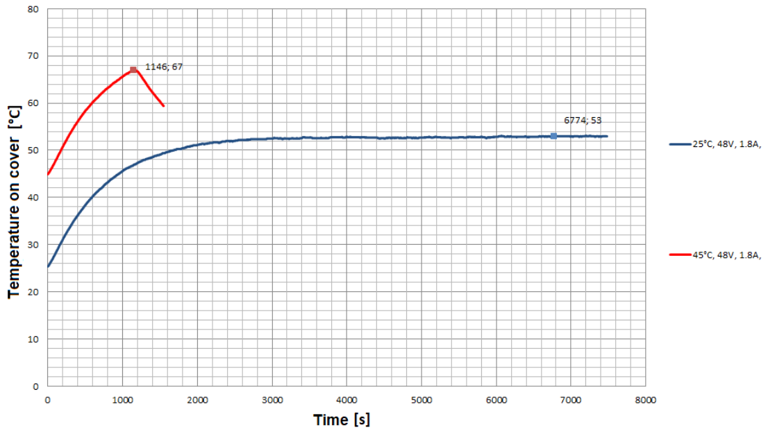
PD2-C Temperature
