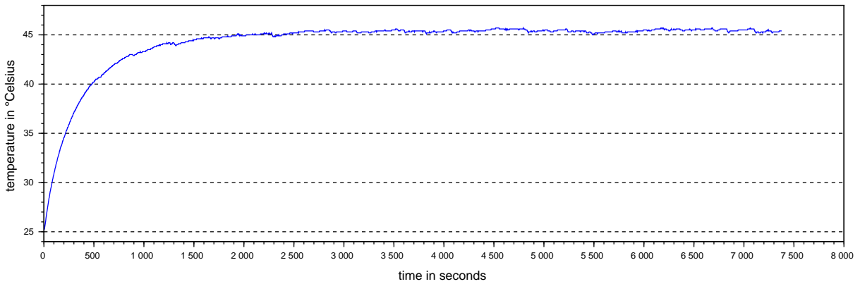
C5: Controller temperature at 25° Celsius ambient temperature and 6A motor current
