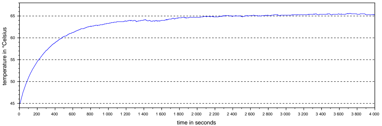
C5: Controller temperature at 45° Celsius ambient temperature and 6A motor current
