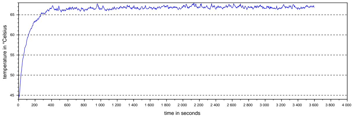
CL3-E: Controller temperature at 45° Celsius ambient temperature and 3A motor current
