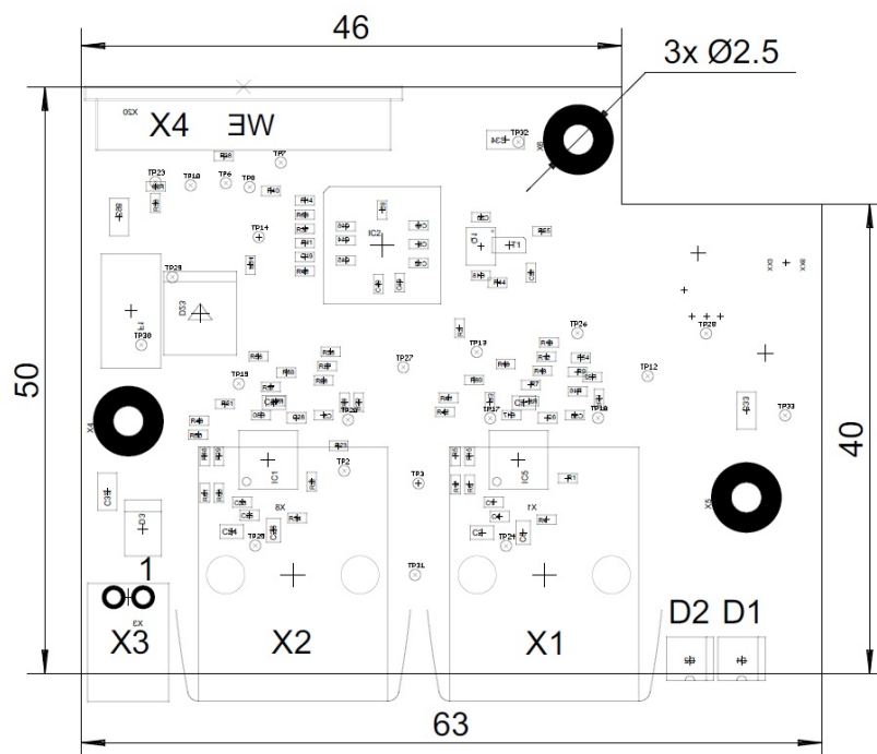
Hardware overview – EtherCAT additional board
