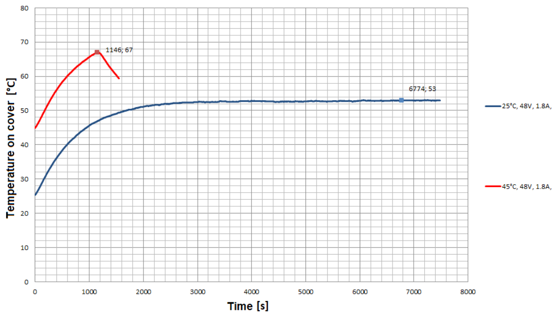
PD2-C Temperature
