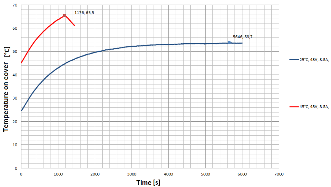
PD2-CB Temperature
