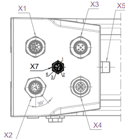
Abb. 3: STO connector X7
