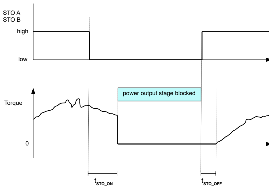
Abb. 2: Activation and deactivation of the STO function
