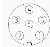
Abb. 4: Pin assignment of the STO connection
