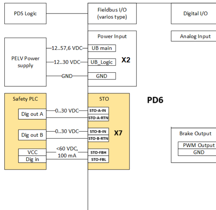
Abb. 5: Wiring example of PD6-E...S-65... for the initial commissioning with the STO function
